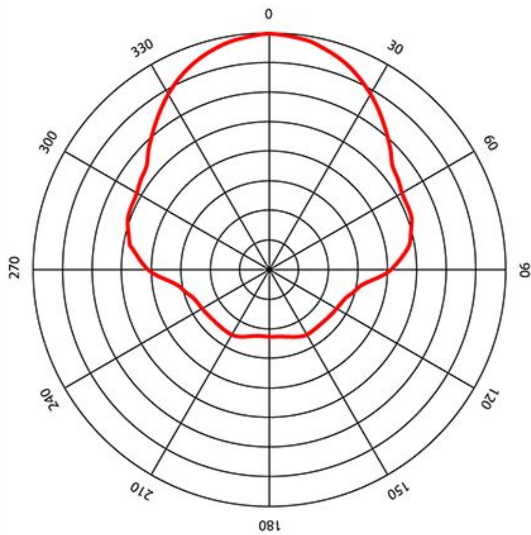
Diameter = 2\lambda
