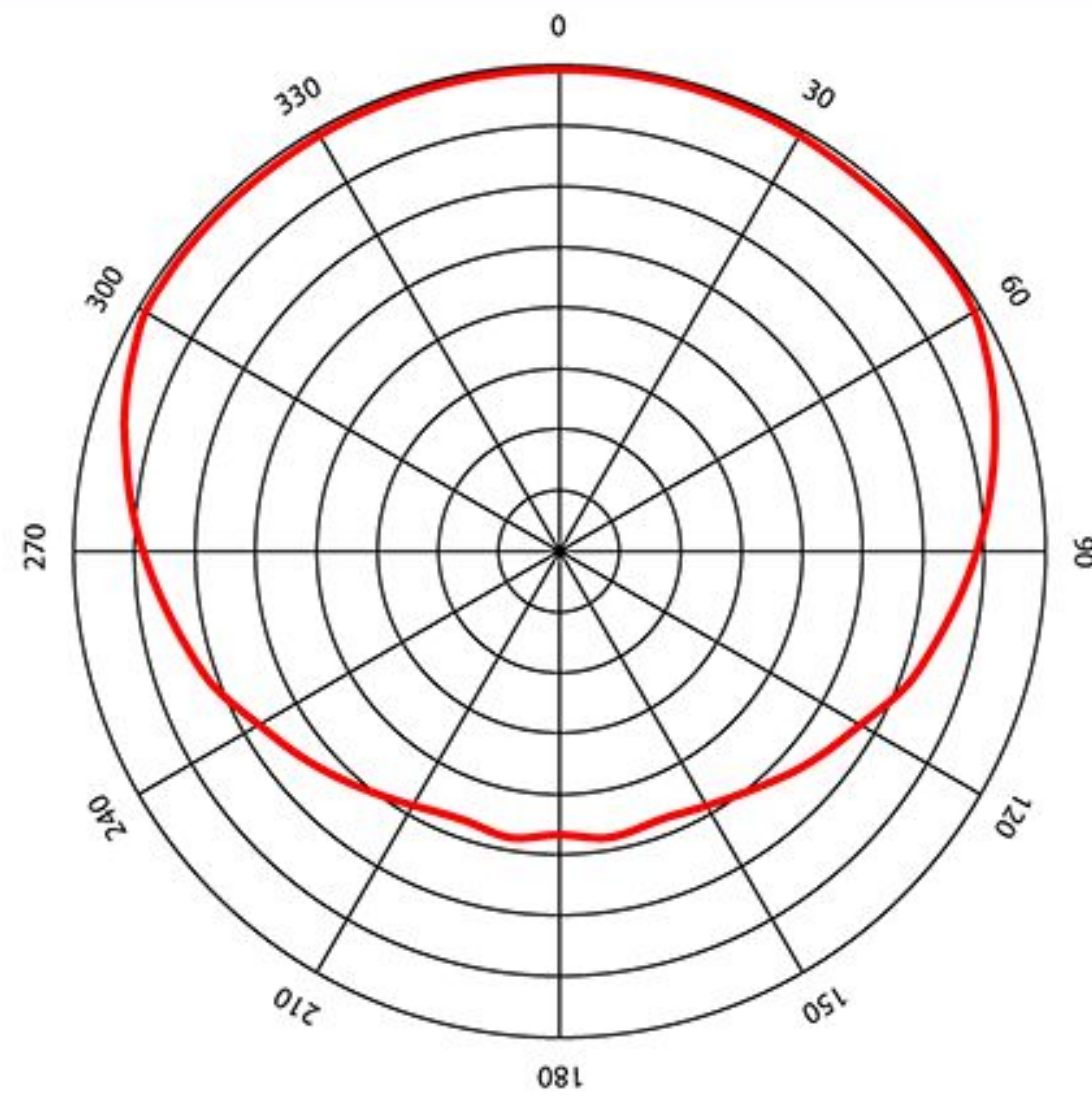
Diameter = 1/2\lambda
