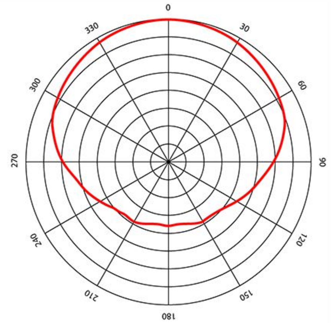
Diameter = \lambda
